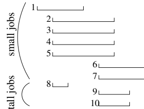
release time deadline intervals
