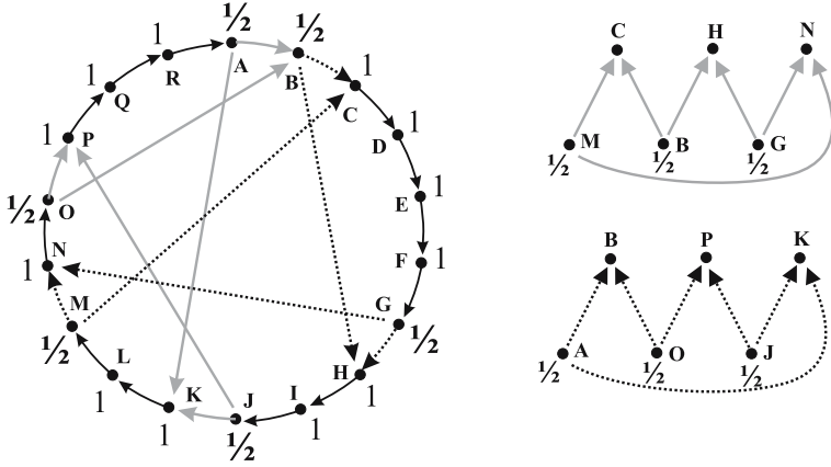
Fig. 7. An example of subgraph obtained after phase 2 and the corresponding weight assignment
