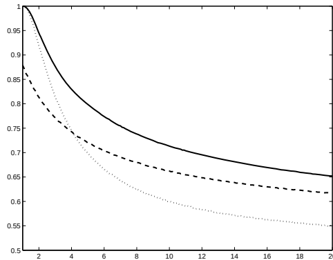
Fig. 2. Our values of the lower bound \text{lb}(d) (solid line), obtained by the numerical solution of differential equations (and corroborated by simulation experiments), juxtaposed with the corresponding values obtained by simulating the algorithms in Coja-Oghlan et al. [6] (dashed line) and Coppersmith et al. [7] (dotted line), for values of average degree d \in [1, 20]
