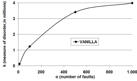
Fig. 1. Disorder produced by random memory faults in the sequence output by VANILLA mergesort. In this experiment n = 5 \cdot 10^6 and \alpha = \delta increases up to 1000.
