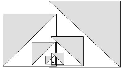
Fig. 1. A guard can be contained in many bounding boxes
