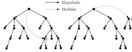
Fig. 2. Consequence due to the greedy user model assumption
