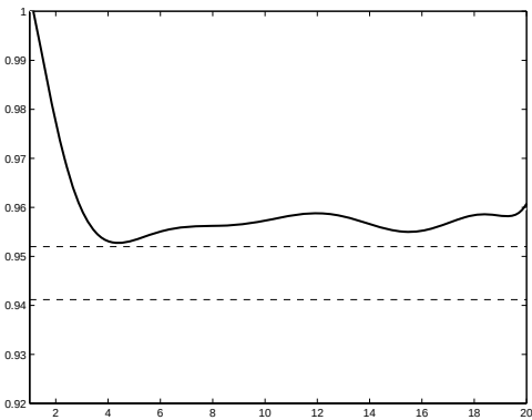
Fig. 3. The approximation ratio \text{lb}(d)/\text{ub}(d) , for values of average degree d \in [1, 20] . The lower dashed line corresponds to Håstad inapproximability threshold 16/17 , while the upper dashed line to our approximation ratio 0.952 .
